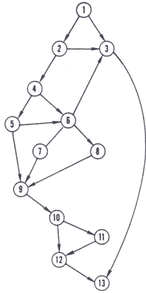
V(G) = 8
