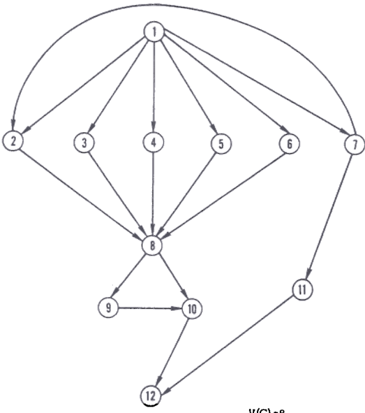
V(G) = 8
