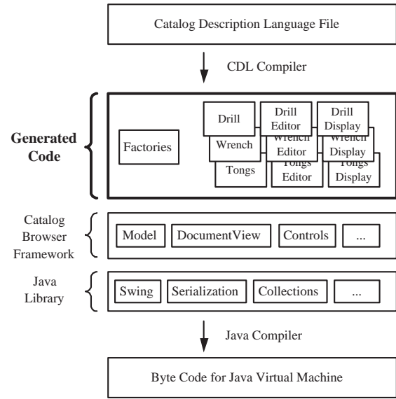
Figure 12. CDL stack
