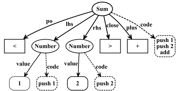
Figure 9. Syntax tree after transformation to postfix notation
