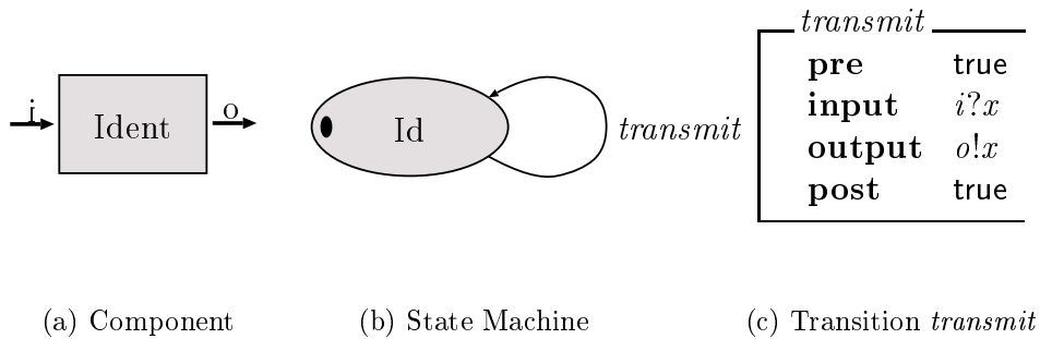
Figure 1: Identity Component
