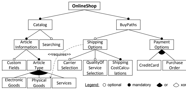
Figure 1. Example feature model for online shops.
