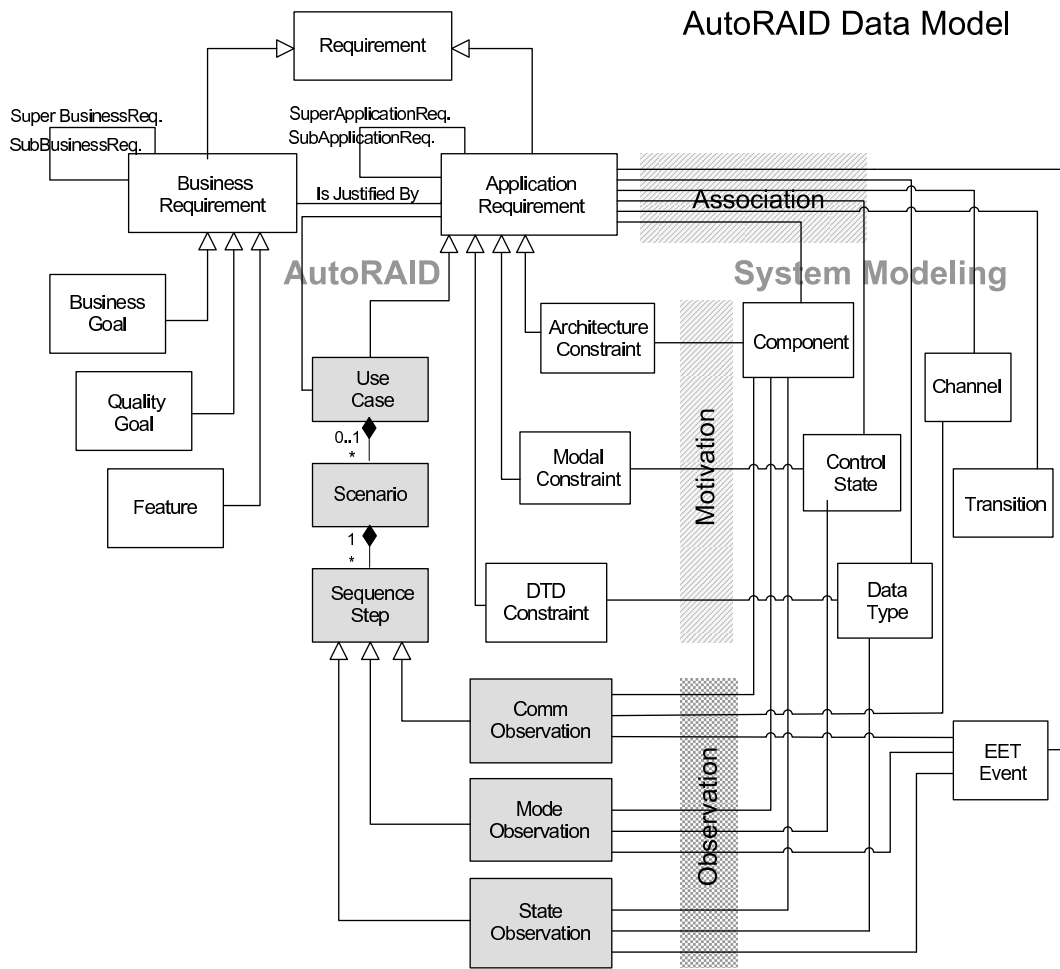
Figure 6. AUTO RAID Data Model
