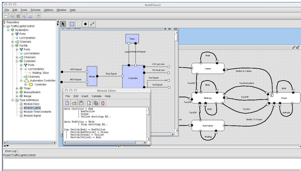
Figure 4. System Views and Representation Techniques in AUTOFOCUS
