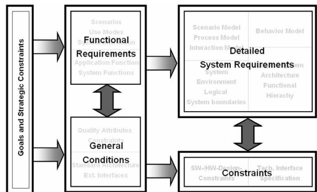
Figure 2. Classification Scheme of Requirements
