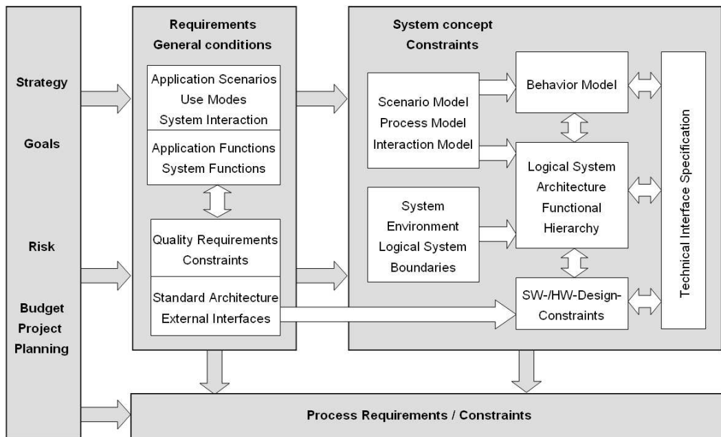
Figure 1. RE Product Model
