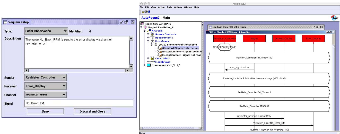
Figure 10. Scenario Analysis in AUTO RAID
