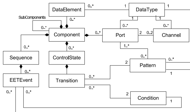
Figure 5. Model Relations in AUTOFOCUS
