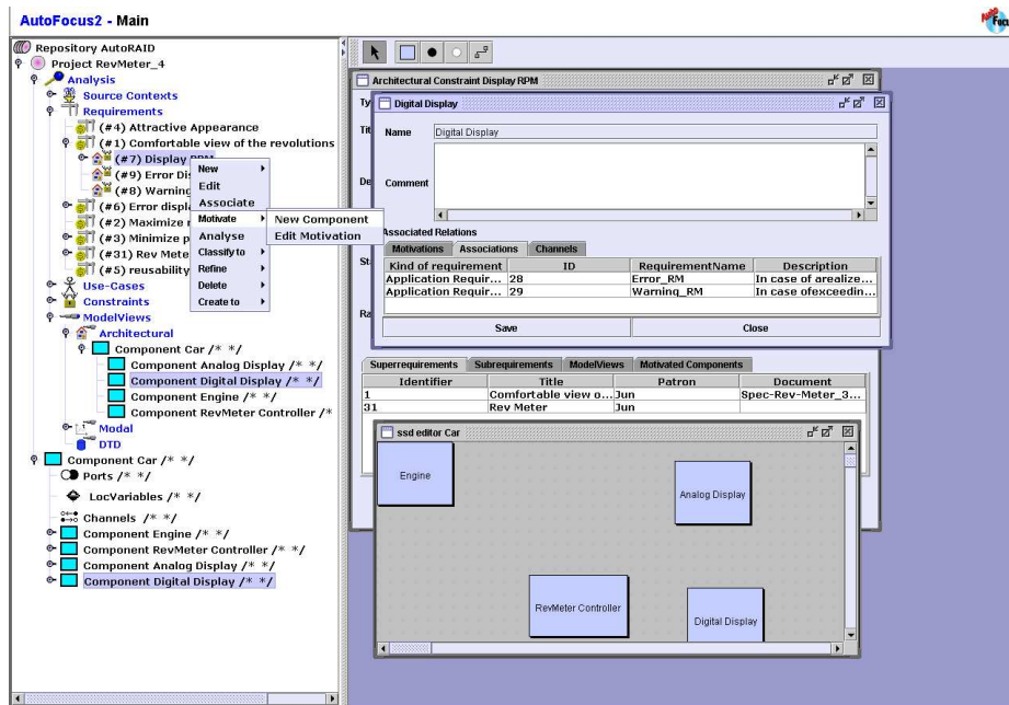
Figure 8. Motivation- and Association-Functions in AUTORAID
