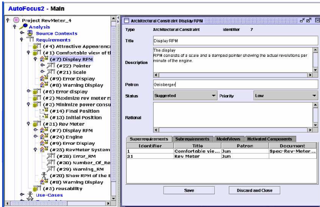
Figure 7. AUTORAID User Interface
