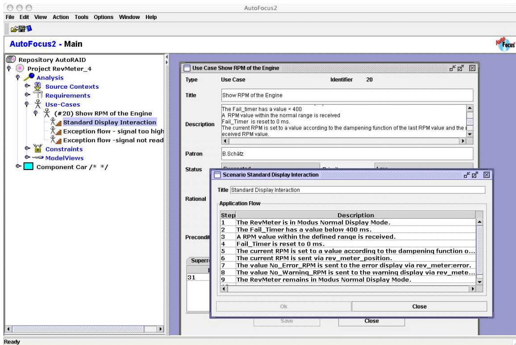
Figure 9. Use Case- and Scenario-Modeling in AUTO RAID
