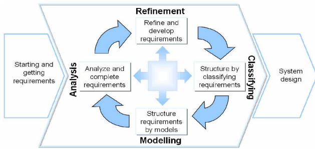
Figure 3. Iterative Process Model in AUTORAID
