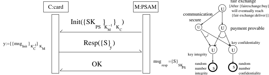
Figure 4: Sequence diagram and goal tree
