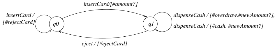
Fig. 9. Lifecycle Automaton
