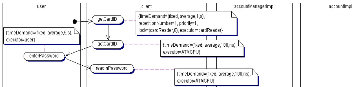
Figure 5: A fragment of the activity diagram constructed for Get_AccountInfo
