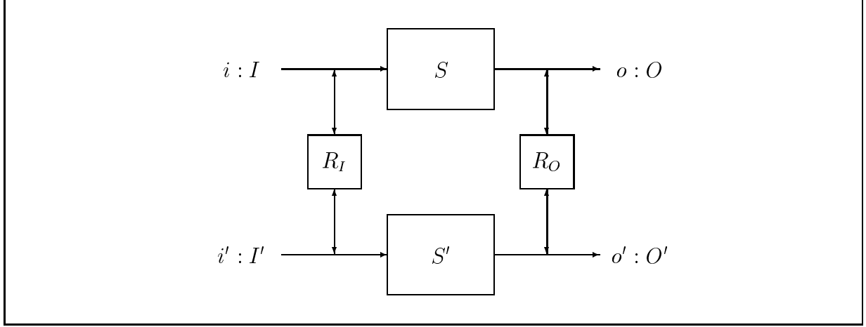
Figure 1: Interaction-Refinement
