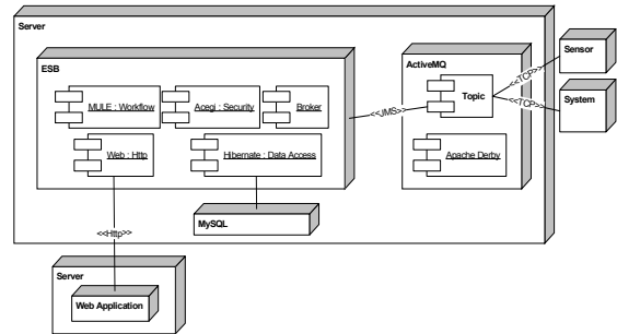
Figure 2. Deployment infrastructure
