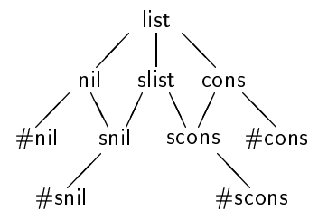
Figure 11: Type hierarchy of the List package
