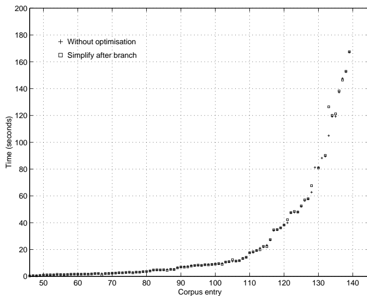
(c) Simplify-after-Branch
