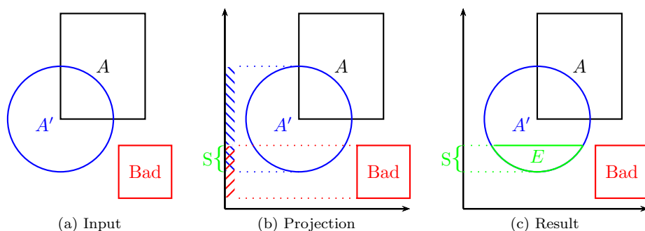
Figure 3.5: \text{Extract}(A, A', \text{Bad})
