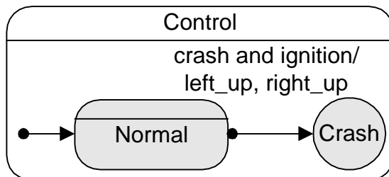
Figure 4: Syncchart Crash Detection—Central Locking System
